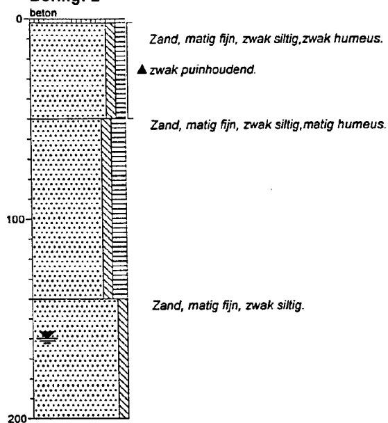
Boring: 2
