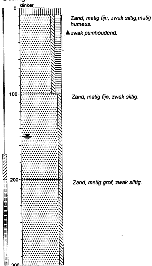
Boring: 1
