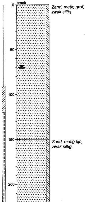
Boring: 1
