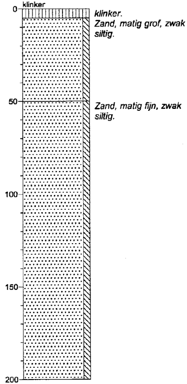
Boring: 2
