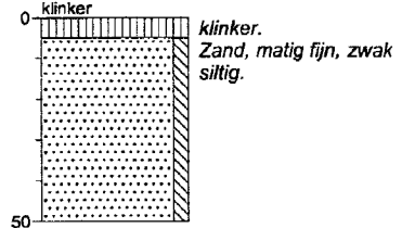
Boring: 3
