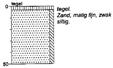
Boring: 8
