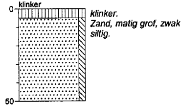
Boring: 5
