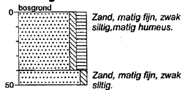
Boring: 5
