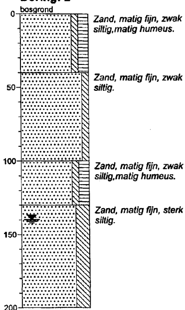
Boring: 2
