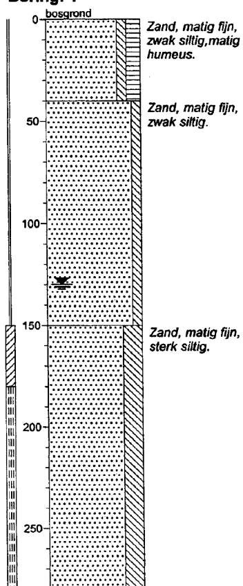
Boring: 1
