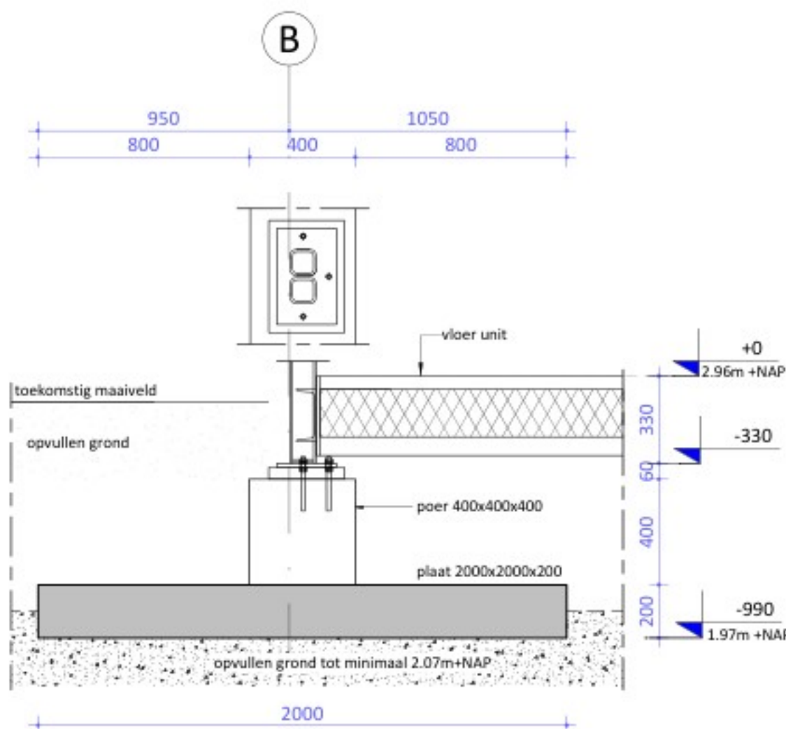
Detail 01
