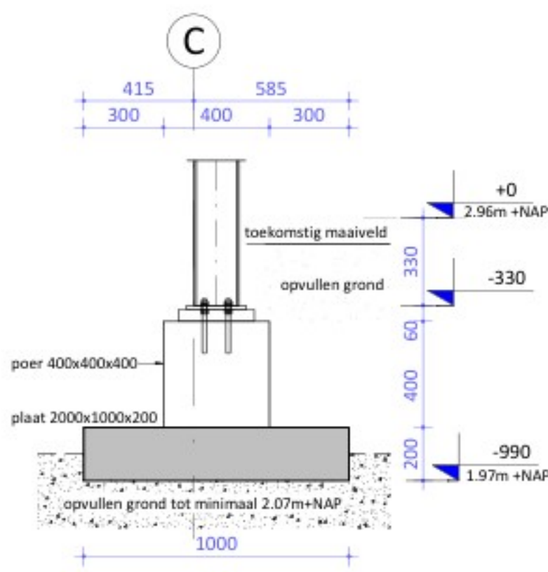
Detail 02
