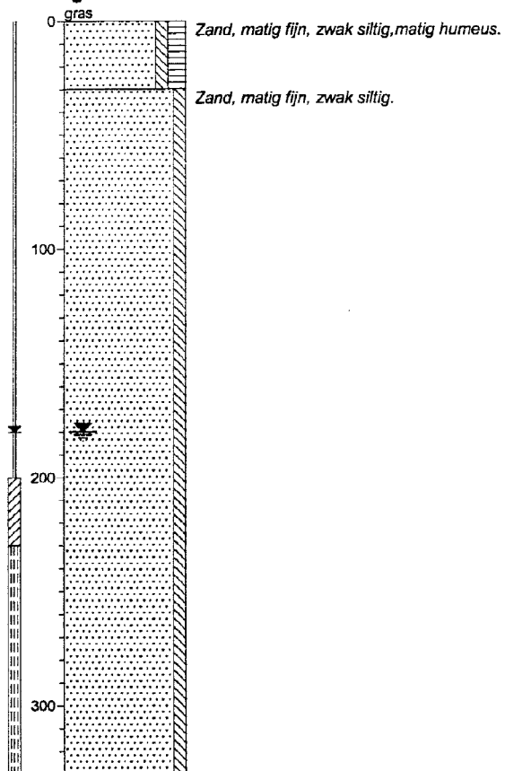
Boring: 1
