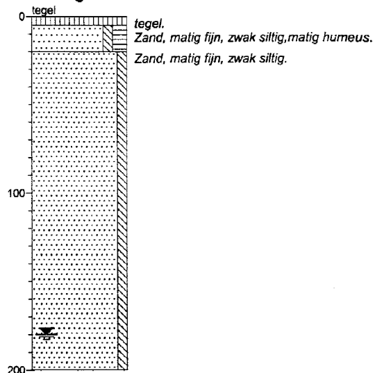
Boring: 2
