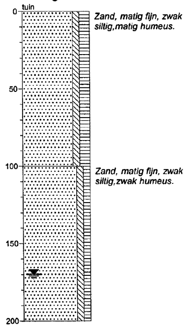
Boring: 6
