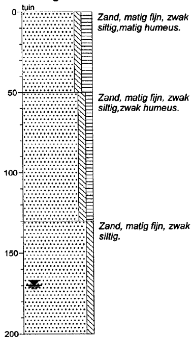
Boring: 4
