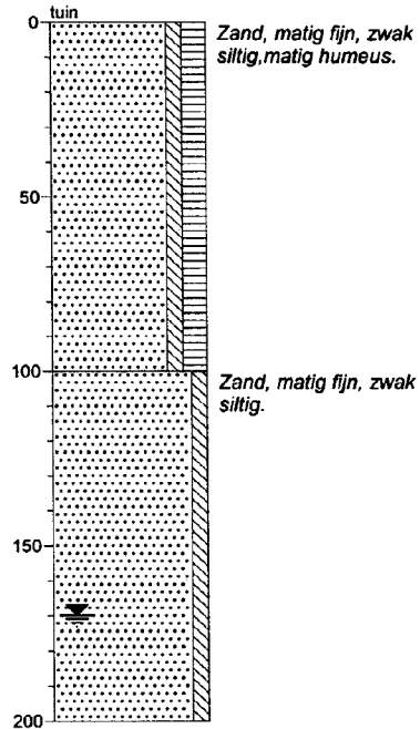
Boring: 10
