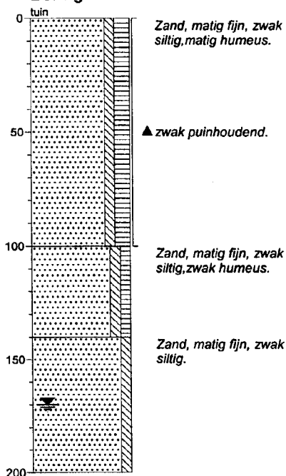
Boring: 1
