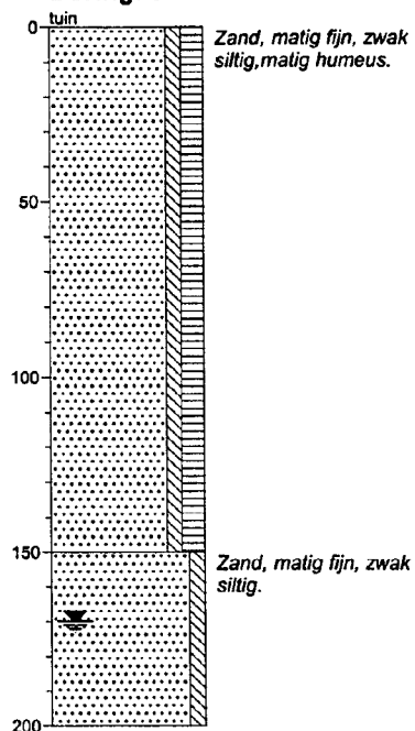
Boring: 9
