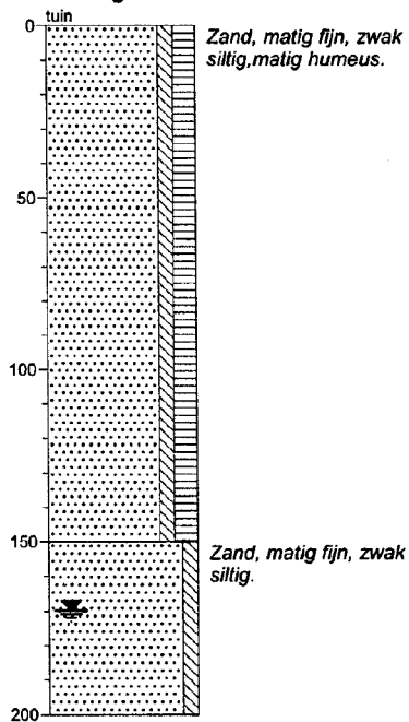
Boring: 5
