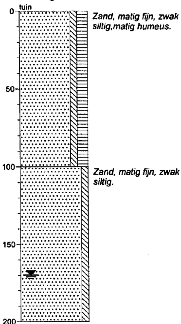
Boring: 7
