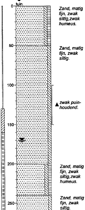
Boring: 8
