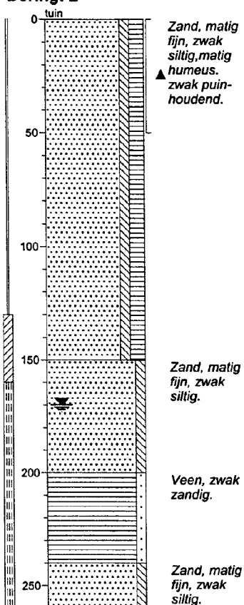
Boring: 2
