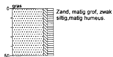
Boring: 6
