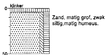
Boring: 5
