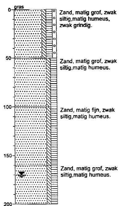
Boring: 2
