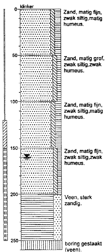
Boring: 1
