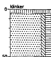
Boring: 7
