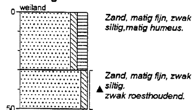
Boring: 12
