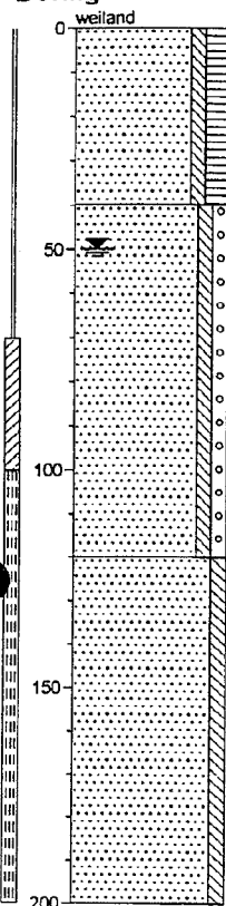
Boring: 1
