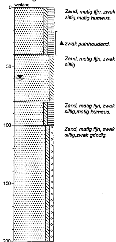
Boring: 8
