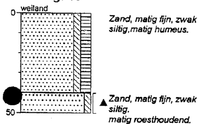
Boring: 10
