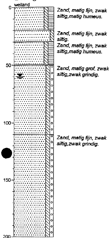
Boring: 7
