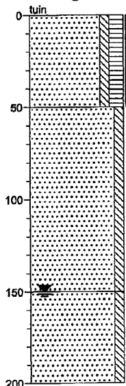
Boring: 2
