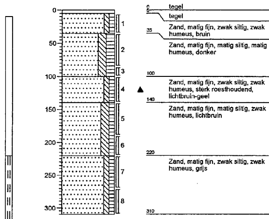
Boring: 3
