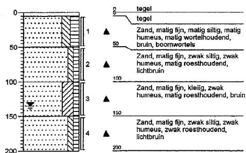
Boring: 5
